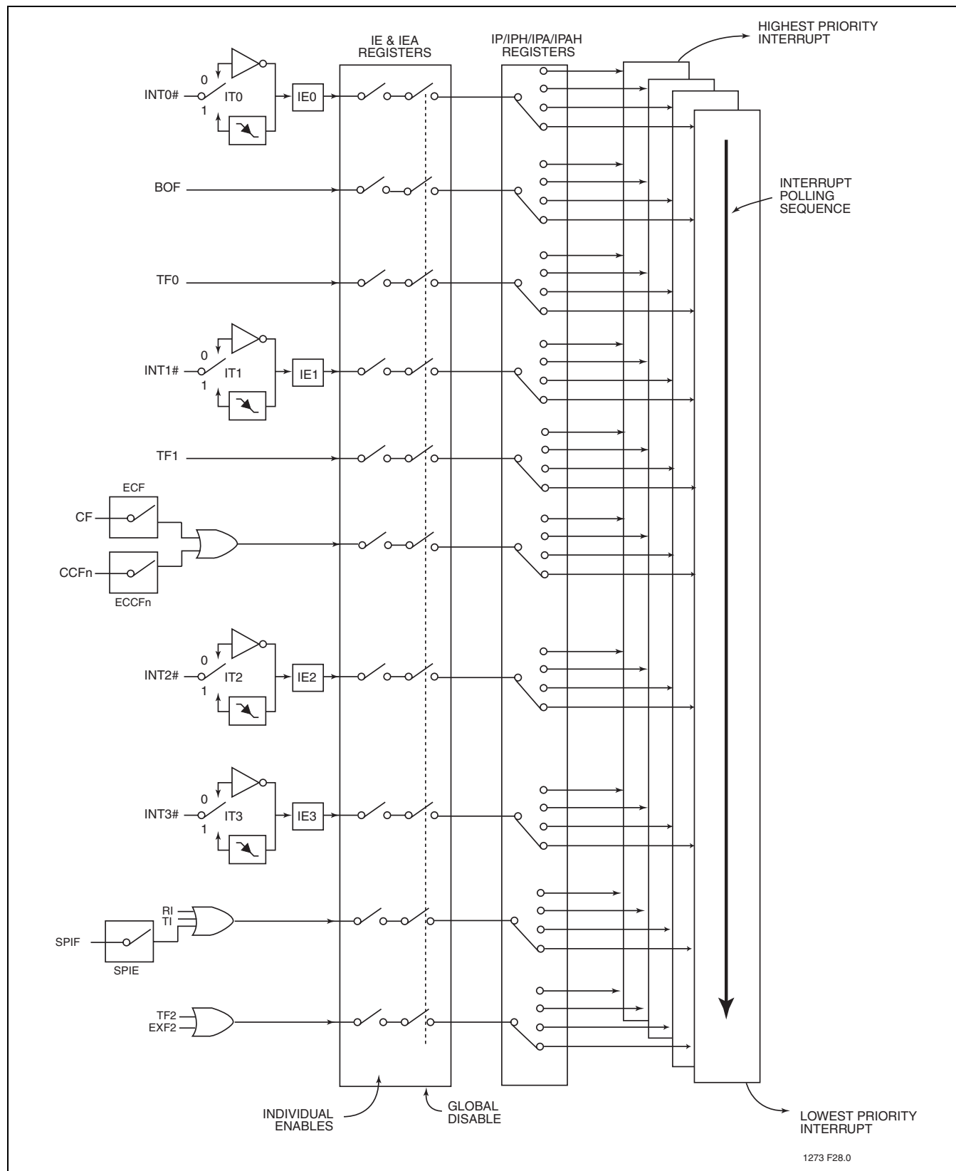
FIGURE 11-1: Interrupt Structure
